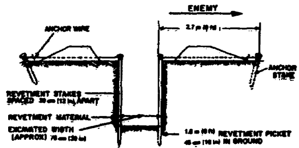
Figure 1-10. Supporting and anchoring revetment.
